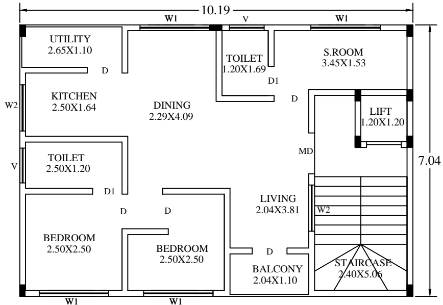
TYP: FIRST & SECOND FLOOR PLAN
