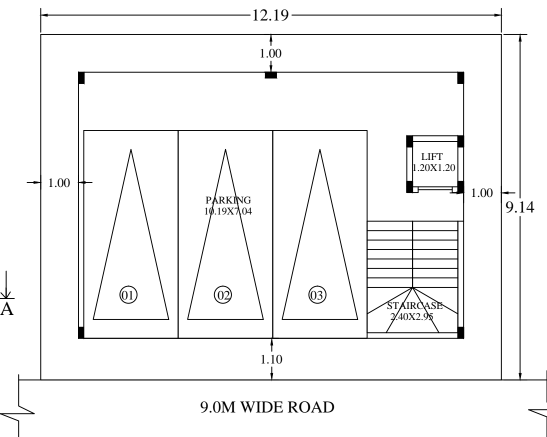
STILT FLOOR PLAN
